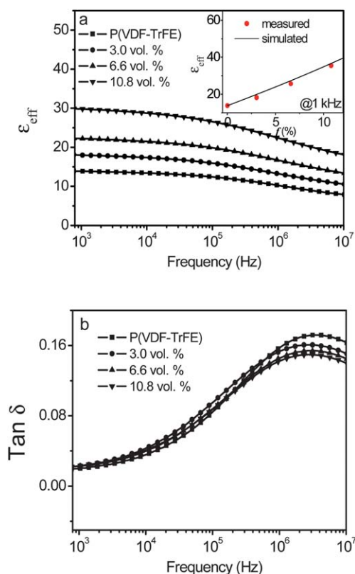
Fig. 3 Dependencies of the dielectric relative permittivity, \epsilon_{\text{eff}} (a) and dielectric loss, \tan \delta (b) at a frequency from 800 Hz to 10 MHz of the BaTiO 3 /PVDF-TrFE nanocomposites with different volume fractions of dopamine modified BaTiO 3 nanofibers. Superimposed in the inset is the dielectric relative permittivity calculated according to eqn (1).
